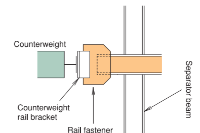
Example of fixing the counterweight rail brackets in A to a separator beam
