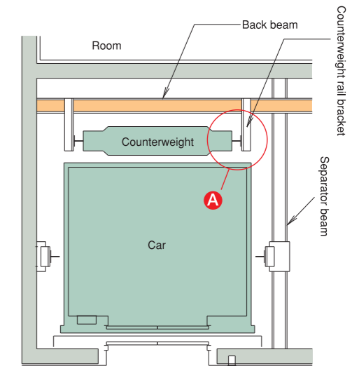
Figure 7 1. When the room is behind the shaft (Back-beam insertion example)
