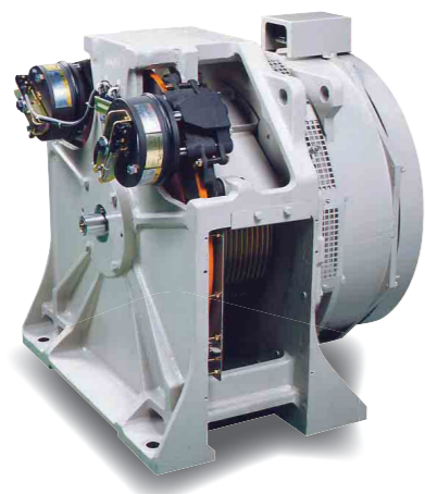
Permanent magnet synchronous motor
