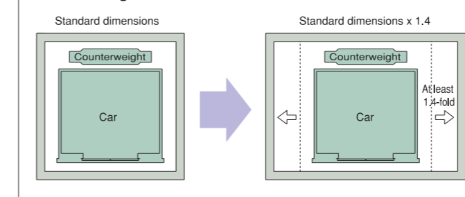
Figure 2. Measures Against Wind Shear
