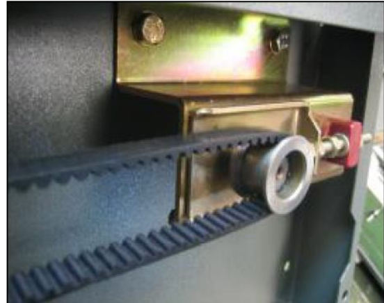
Idle Pulley Tensioner & Support For RAC 250 Operator (left hand side view)
