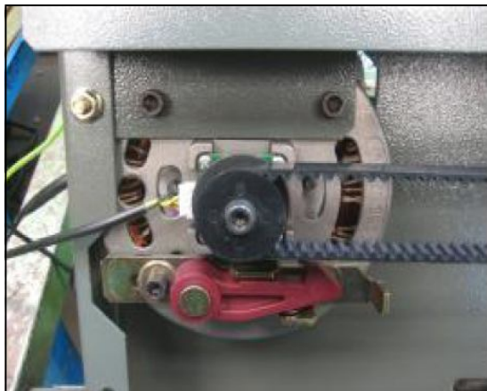
Stopping Retainer Assembly For RAC 250 Operator
