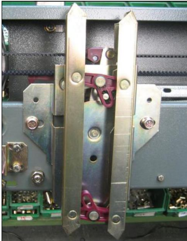
Skate For RAC 250 Operator
